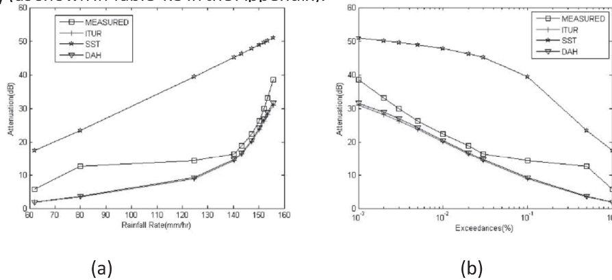
FIG 4.6 Comparison of attenuation values against (a) rainfall rate (b) percentage time Marina at 12GHz Figures 4.6 and 4.7 shows the plots of the attenuation exceedances for ITU-R, SST and DAH prediction
