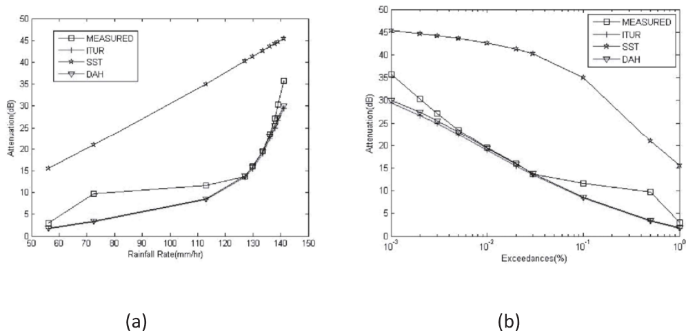
FIG 4.2 Comparison of attenuation values against (a) rainfall rate (b) percentage time for Ikeja at 12GHz.
