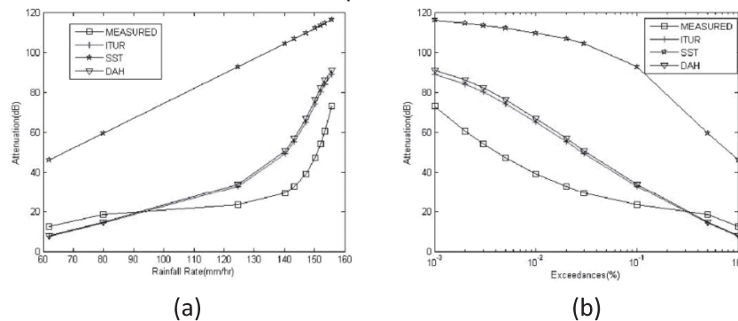
FIG 4.7 Comparison of attenuation values against (a) rainfall rate (b) percentage time Marina at 23GHz
