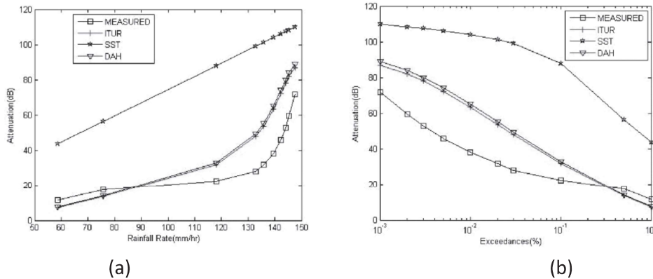
FIG 4.5 Comparison of attenuation values against (a) rainfall rate (b) percentage time for Oshodi at 23GHz
