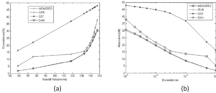
FIG 4.4 Comparison of attenuation values against (a) rainfall rate (b) percentage time for Oshodi at 12GHz
