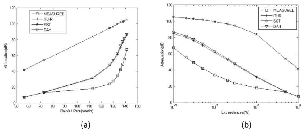
FIG 4.3 Comparison of attenuation values against (a) rainfall rate (b) percentage time for Ikeja at 23 GHz.
